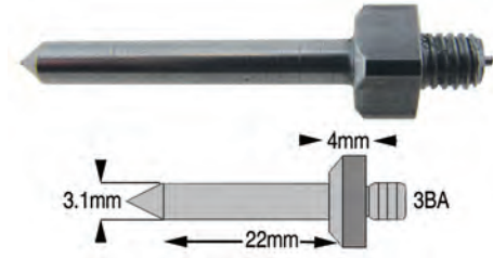
Long Case Clock - Rack Hook & Lifting Piece Stud
