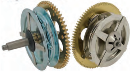
Hermle Strike Side Chain Wheels
